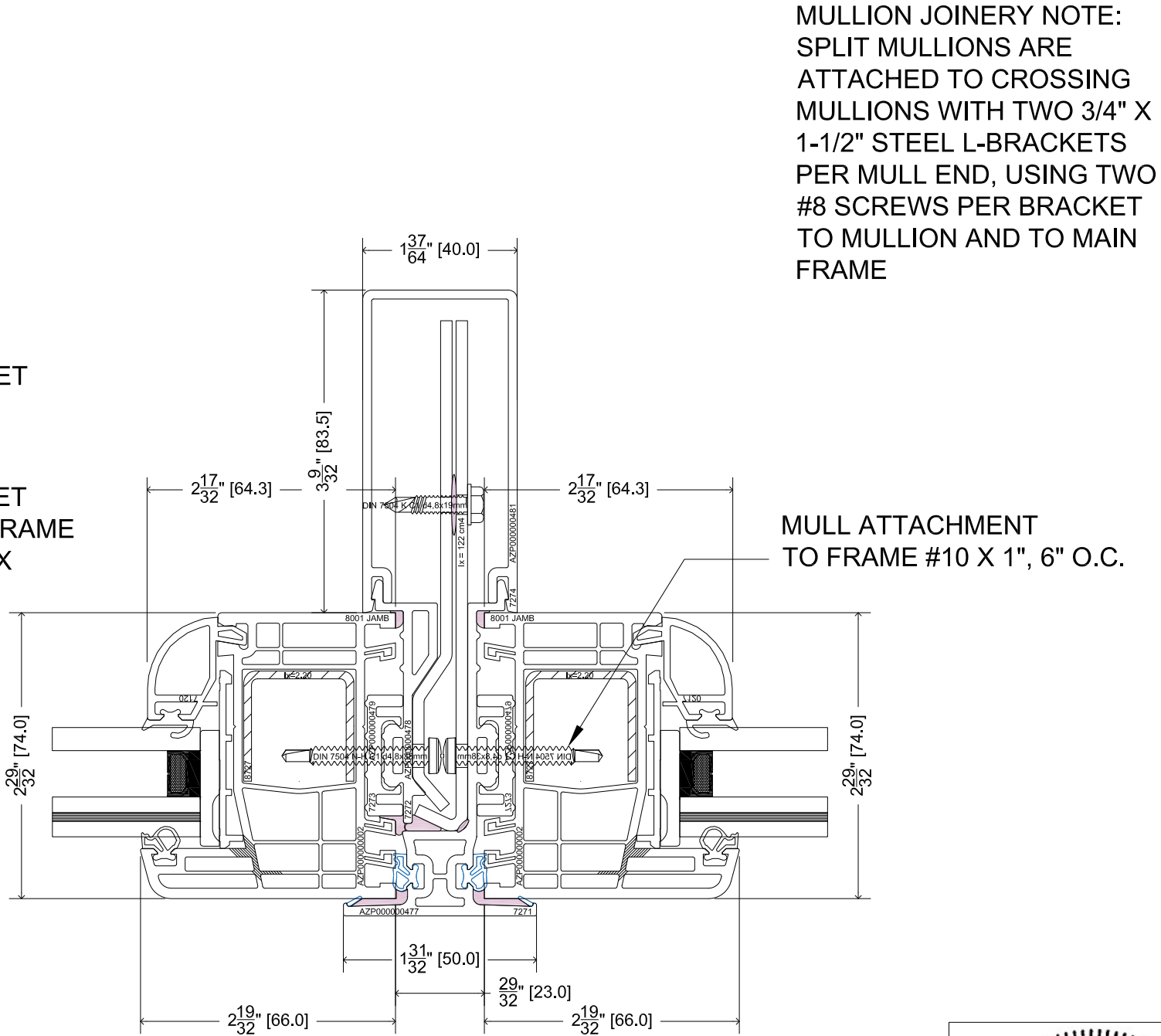
6 TYPICAL SECTION DETAIL PARTIAL VERTICAL MULLION
