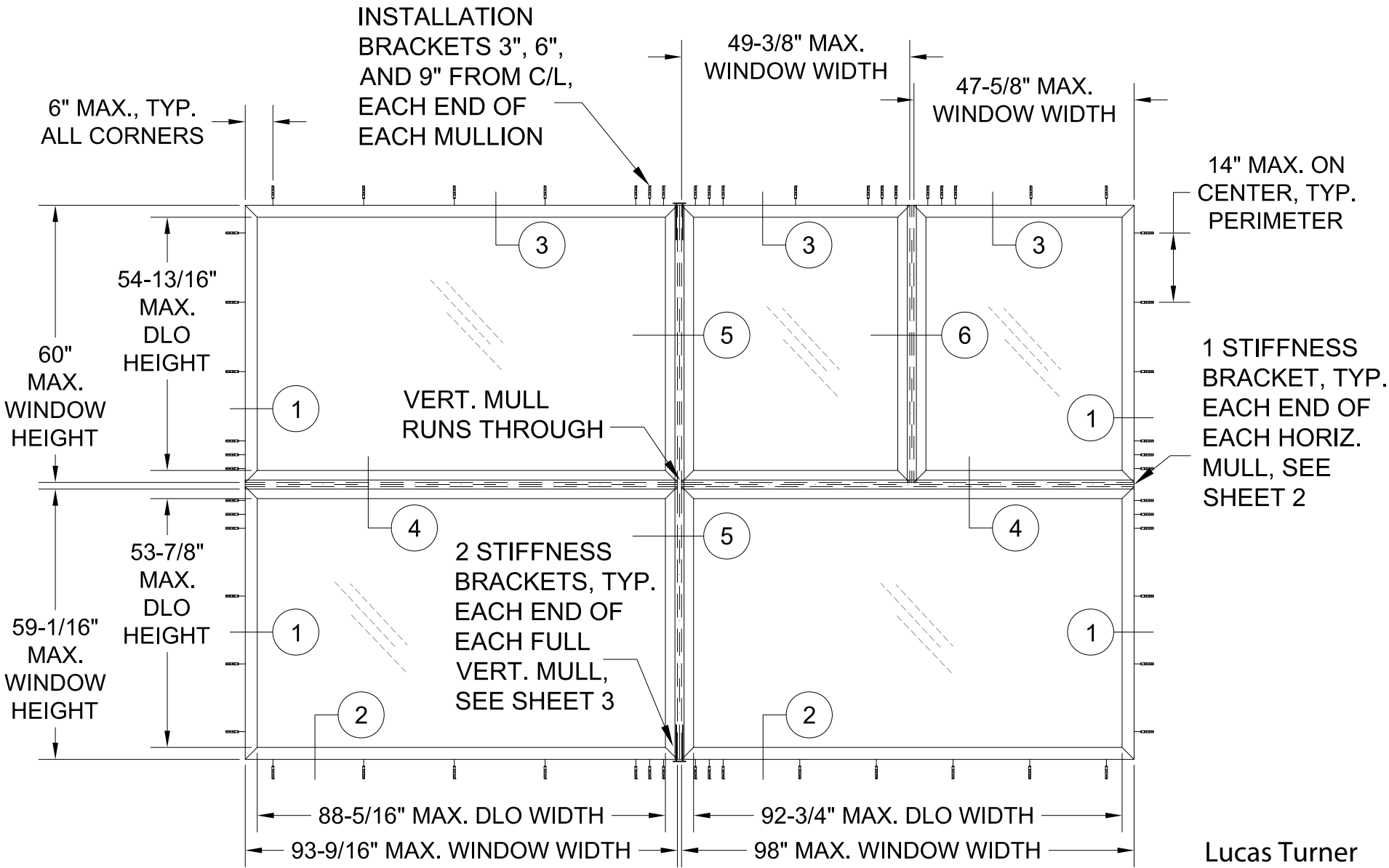
TYP. ELEVATION SEE DETAILS SHEET 2
