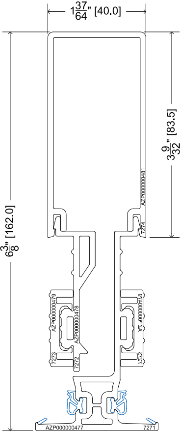
MULLION ASSEMBLY
