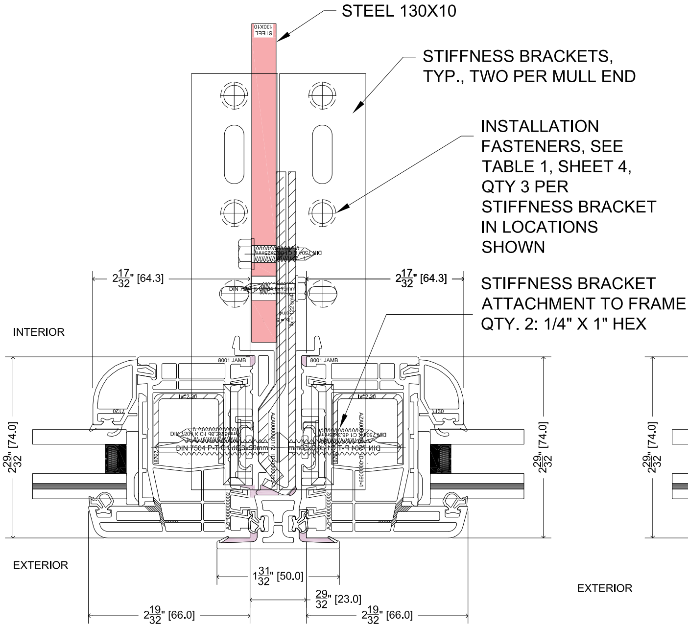
5 TYPICAL SECTION DETAIL FULL VERTICAL MULLION
